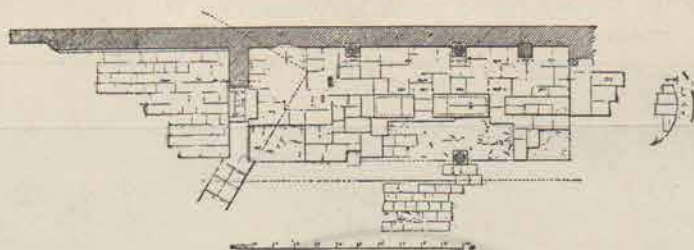
Εἰκ. 138. Ἀρχιτεκτονικὴ κατὰψις τοῦ Ναοῦ Γ (κατὰ τὸν Bohn).
